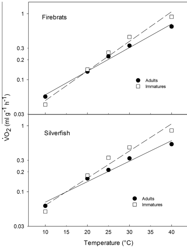
Fig. 1. Mass specific \dot{V}_{O_2} for adult and immature firebrats and silverfish across a range of temperatures. See text for equations.
