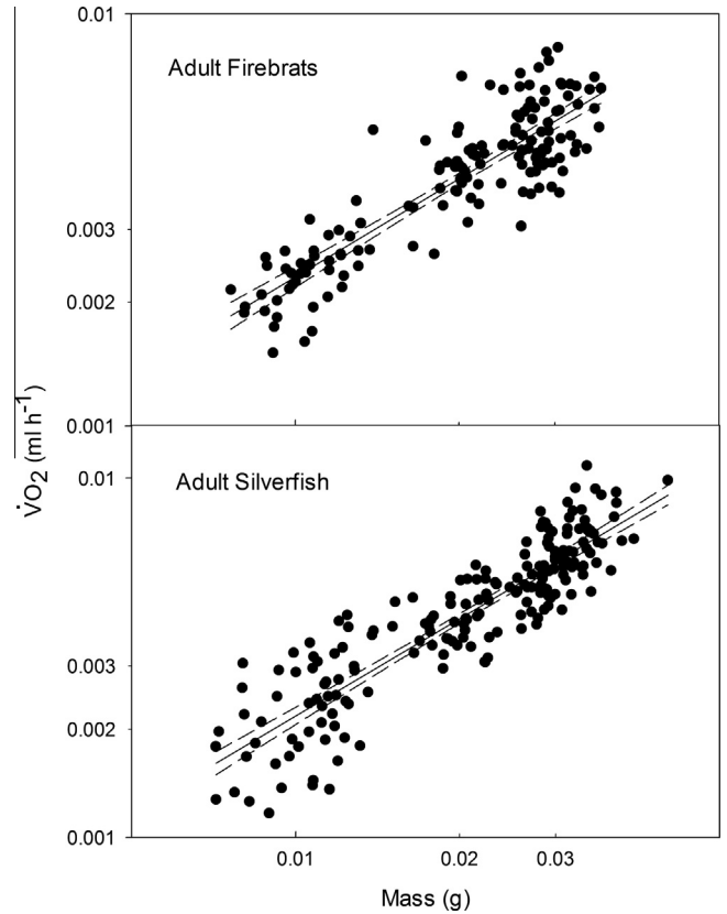
Fig. 2. Temperature adjusted \dot{V}_{O_2} for a range of masses of adult firebrats and silverfish. See text for equations.
